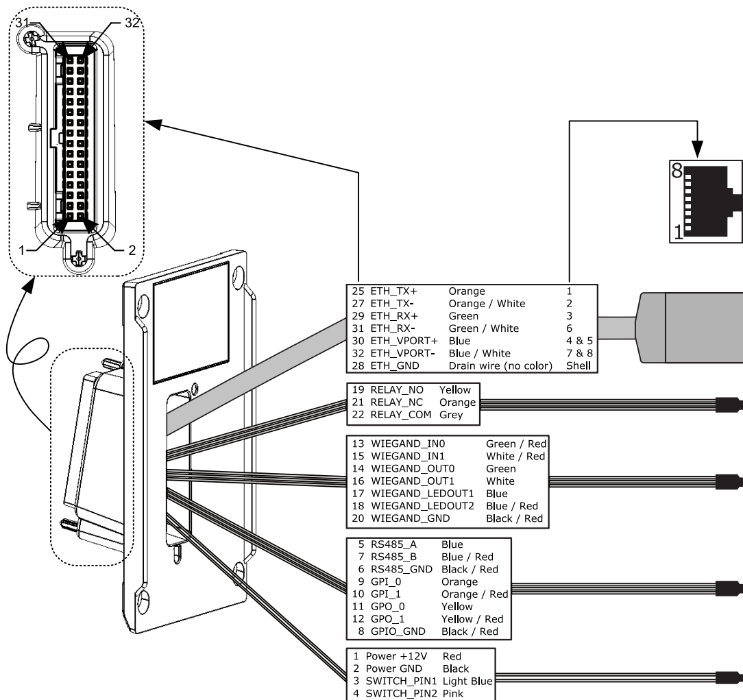
Figure 9: Cabling layout
